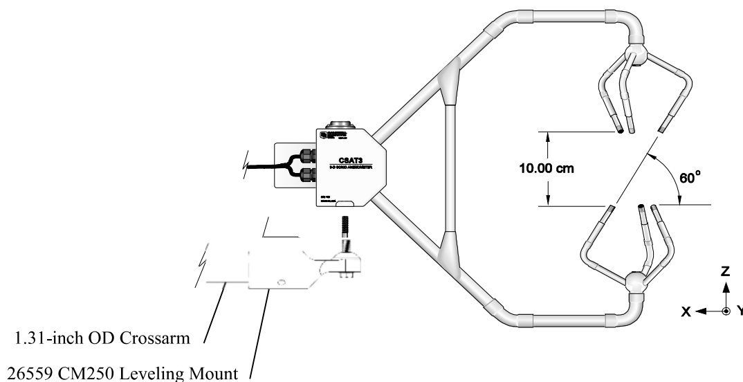
FIGURE 4-1. CSAT3 coordinate system and current captive mounting hardware (s/n 0631 to current)
