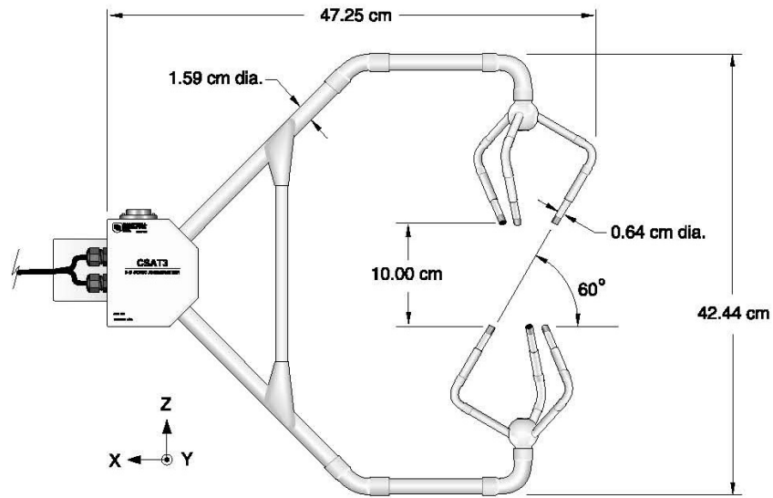
Anemometer Head
